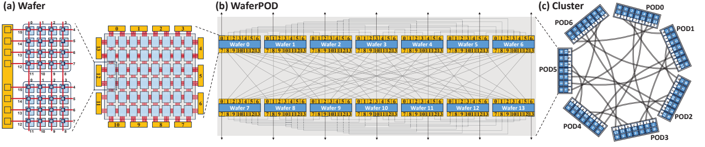
Fig. 8. Switchless dragonfly interconnect across three scales. (a) A wafer aggregates edge links into 14 WCs. (b) A WaferPOD connects 14 wafers in an all-to-all using WCs. (c) Seven WaferPODs form a 98-wafer cluster, where paired outward WCs form PCs.
