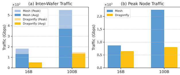
Fig. 15. Impact of interconnect topology on inter-wafer and peak node traffic.
