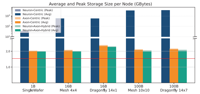
Fig. 14. Memory usage across processing paradigms.
